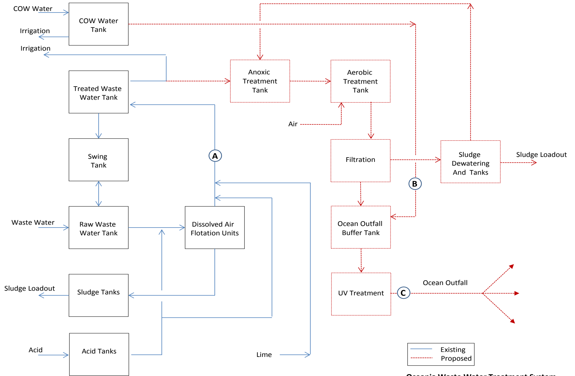
Oceania Waste Water Treatment System
