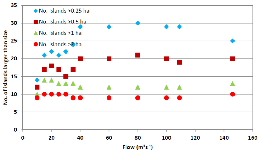
Figure 2. Relationship between flow and number of islands greater than threshold sizes for the Waiau River downstream of Leslie Hills bridge (Source: Duncan 2012).
