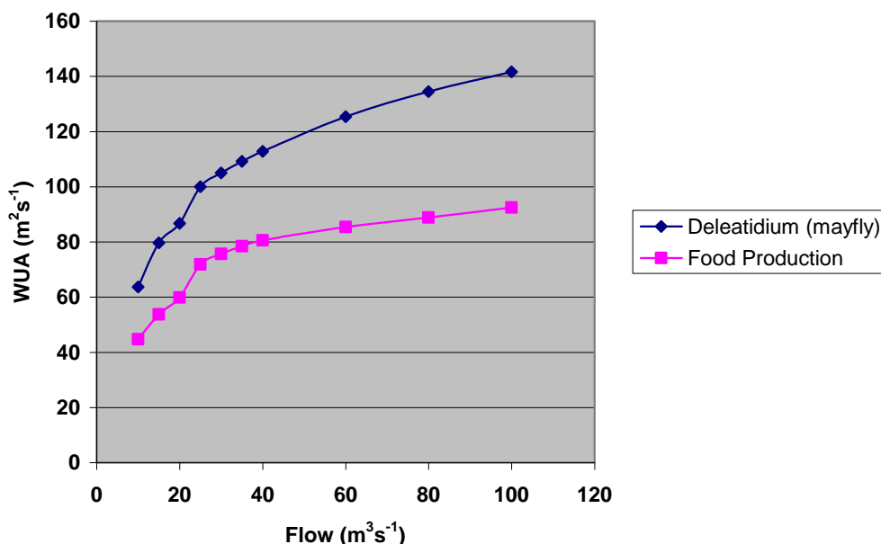
Figure 4. WUA vs modelled flow for benthic invertebrate food production – Waiau River (Source: Duncan and Bind 2009)
