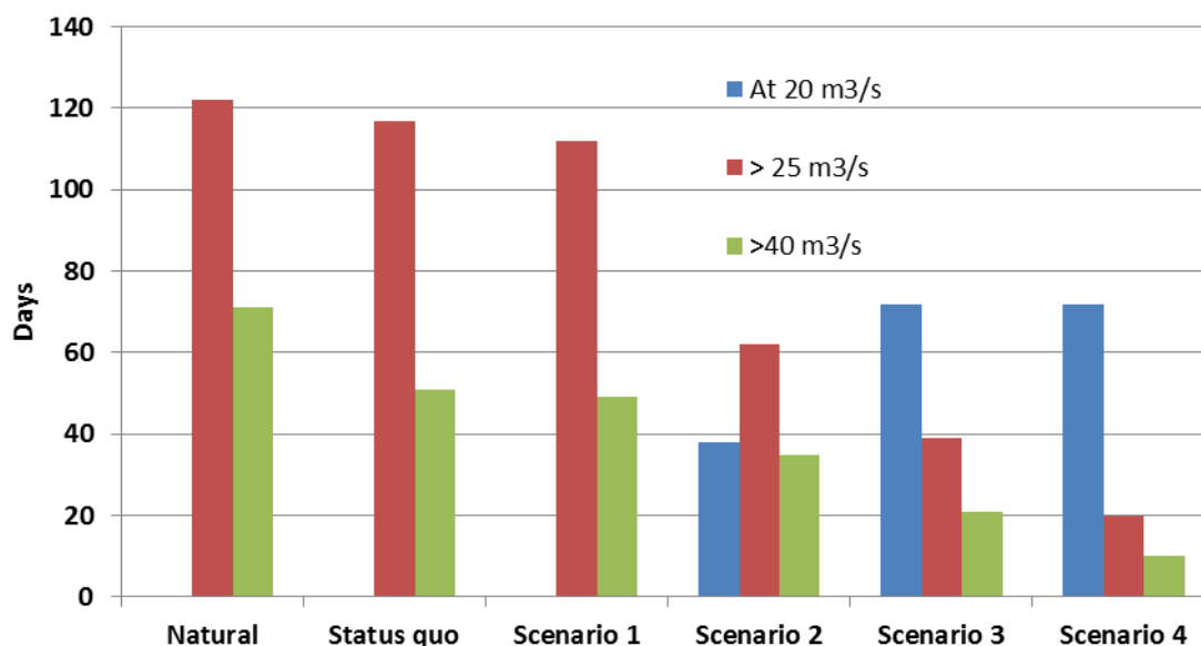
Figure 13. Time during September to December (122 days) when flows are at the minimum or above critical levels in a dry year (Note: green is good and blue is bad for nesting) (Source: Duncan 2012).
