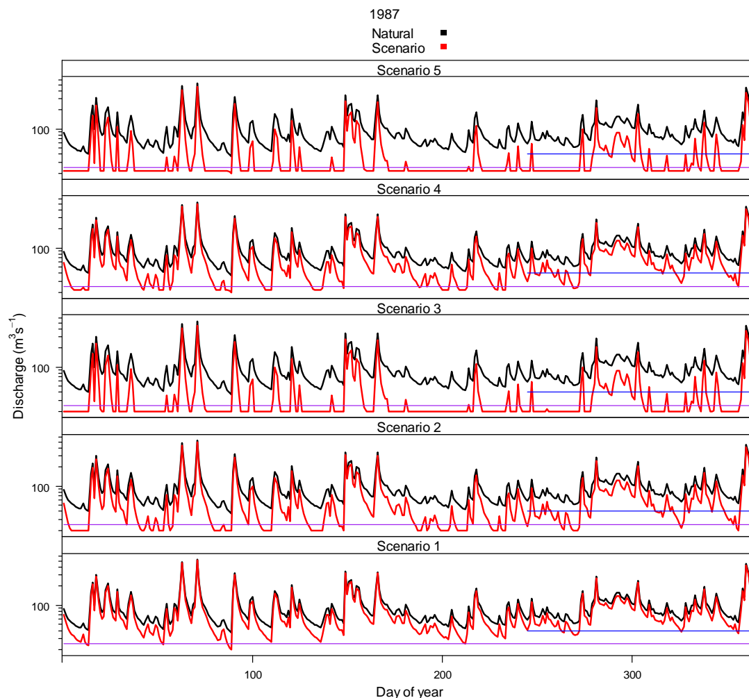
Figure 5. Flow hydrographs for the Waiau River in a typical year (1987). Plots show the natural flow hydrograph (black) and the simulated hydrographs (red) for each of the five management scenarios – note: the blue horizontal line is the best for nesting flow ( 40 \text{ m}^3/\text{s} ) and the purple horizontal line is the best flow for feeding and food production ( 25 \text{ m}^3/\text{s} ). Note that the vertical axis (discharge) is a log scale (Source: Snelder pers. comm. 2012).
