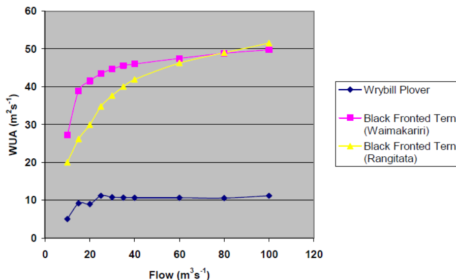
Figure 3. Weighted Usable Area (WUA) vs modelled flow for bird feeding/prey – Waiau River. The Rangitata (Hughey 2001) black-fronted tern curve is for feeding on invertebrates; the Waimakariri (Duncan et al. 2003) curve is for feeding on fish (Source: Duncan 2012).
