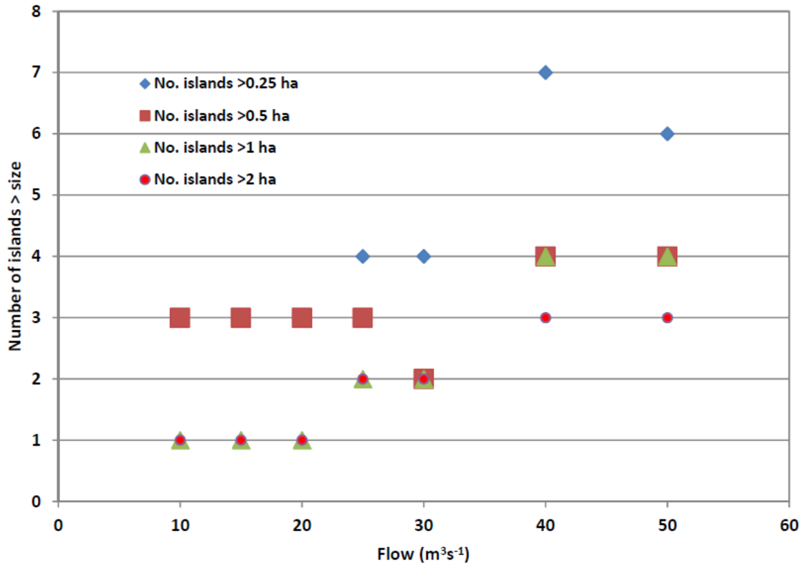
Figure 7. Relationship between flow and number of islands greater than threshold sizes for the Hurunui River downstream of SH6 (Source: Duncan 2012)
