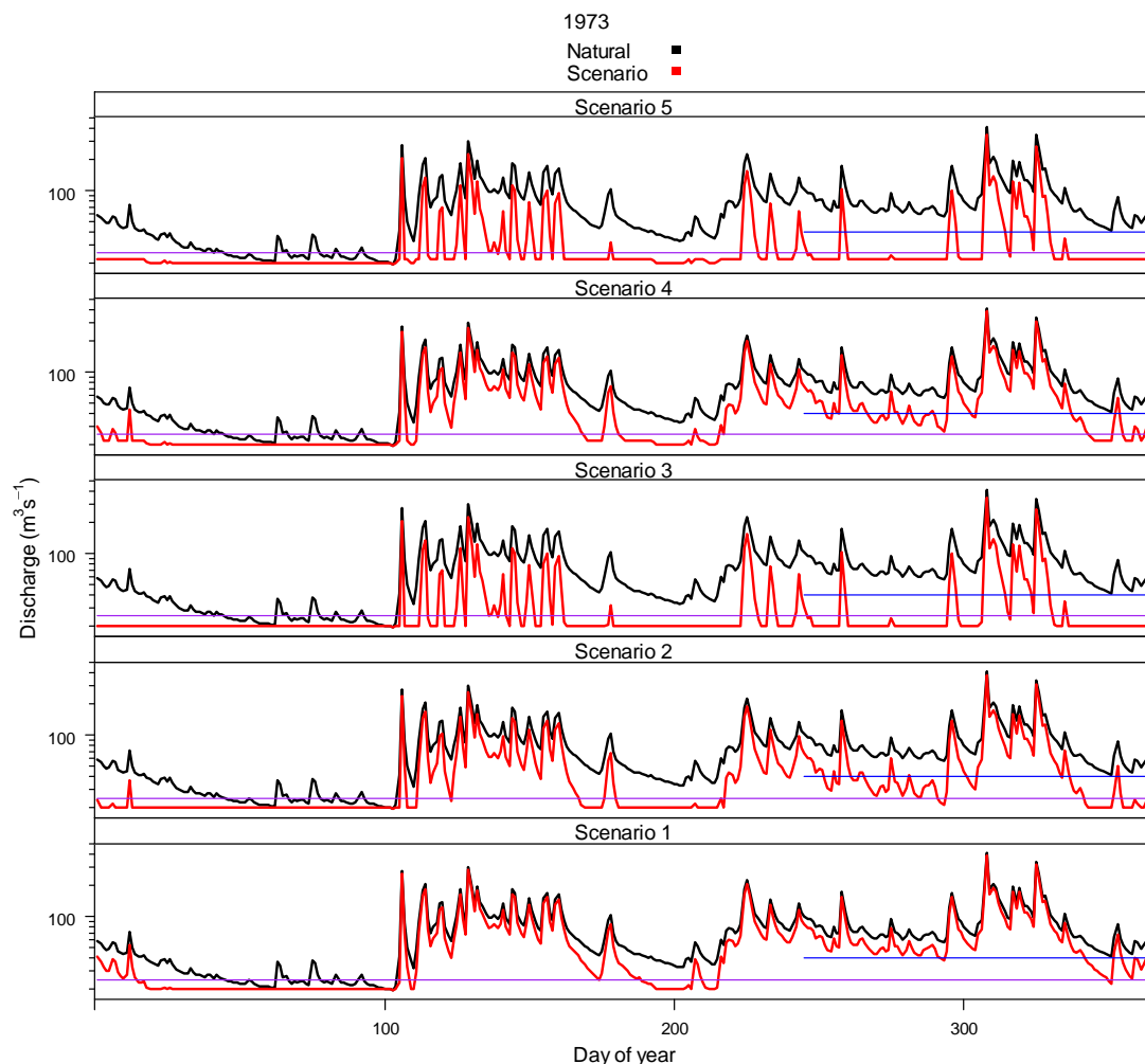
Figure 6. Hydrographs for Waiau River in a dry year (1973). Plots show the natural flow hydrograph (black) and the simulated hydrographs (red) for each of the five management scenarios – note: the blue horizontal line is the best for nesting flow (40 m 3 /s) and the purple horizontal line is the best flow for feeding and food production (25 m 3 /s). Note that the vertical axis (discharge) is a log scale (Source: Snelder pers. comm. 2012).
